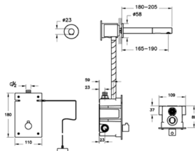
Variable spout length
